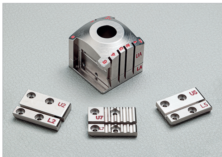
Optional V3 clamp fits interchangeable jaws
